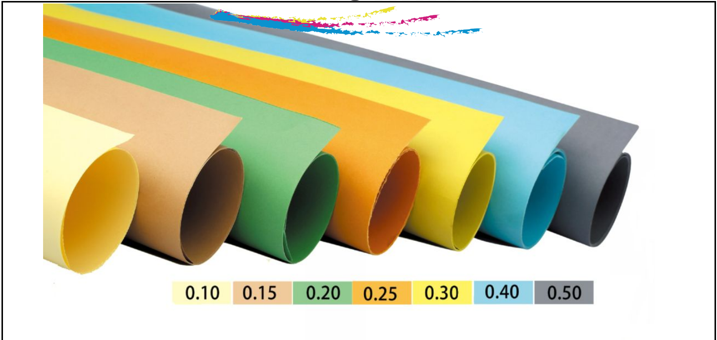
Underpacking paper for under the offset impression cylinder (Tickness Sheetsize)
